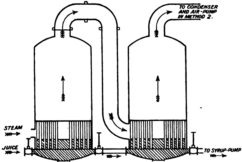
FIG. 23.—DOUBLE-EFFECT EVAPORATOR (Vertical Section)
